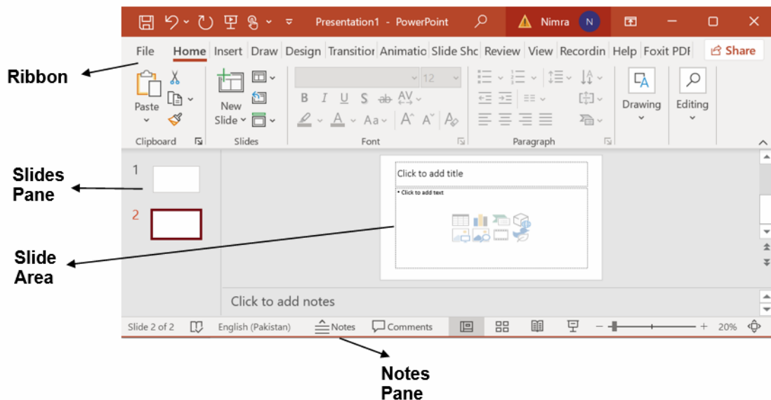
Figure 5: PowerPoint Slide
